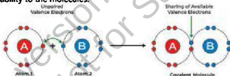
Figure 4.1: Covalent bond between two atoms
